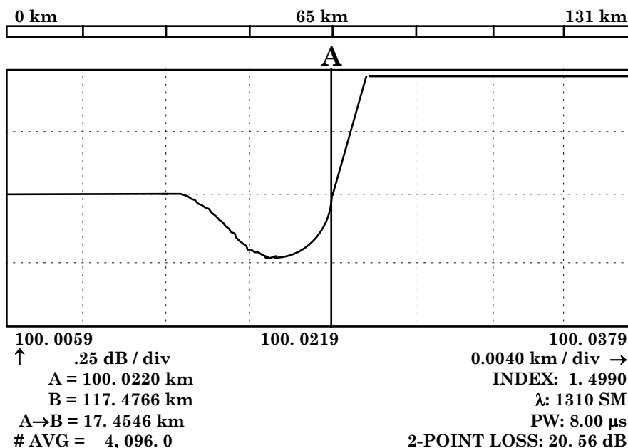
Figure 6. Example of cursor placement if undershoot is present (TD-285C).
